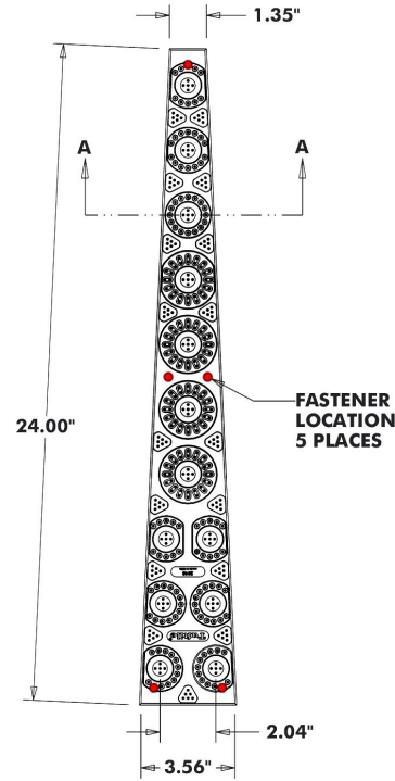
RADIUS - WEDGE TILE
