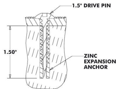
EXPANSION ANCHOR DETAIL (HARDENED CONCRETE)
